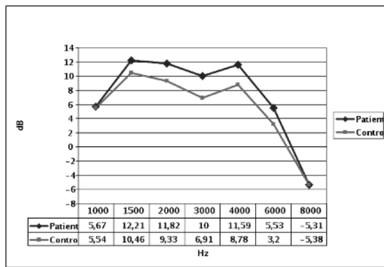
Figure 1. SNR Findings.
